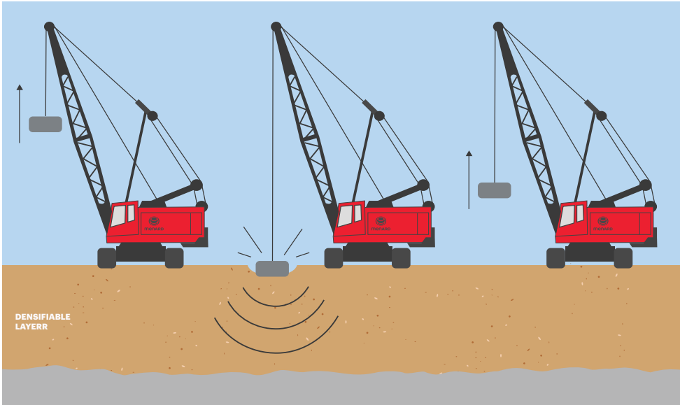
Dynamic Compaction is performed by repeatedly dropping heavy weights on the ground in a predetermined grid pattern
